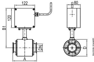
TriClamp®, wall mounted
