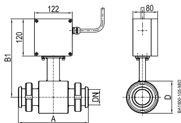
DIN11851, wall mounted
