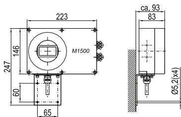
TriClamp®, remote version
